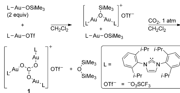
Scheme 1. Preparation of a cationic trigold(I) carbonate.
